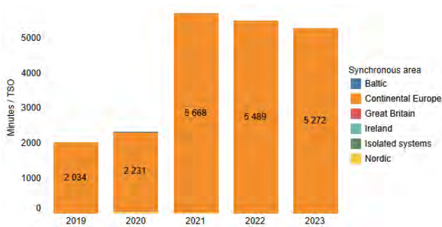
Figure 5.8: Operational security indicator OS-F1 from 2019–2023. It is calculated by adding up the duration of OVBS-, OV0-, OV1- and OV2-incidents and the duration of all other incidents on below scale and scale 0–3 where voltage deviations exceed the ranges from SO GL Annex II [2] are reported, and dividing by the number of TSOs in the synchronous area.
