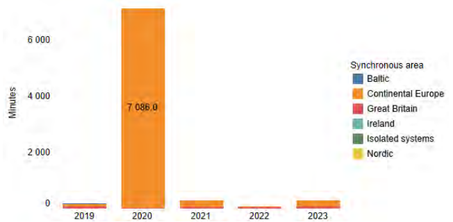
Figure 5.11: Operational security indicator OS-G2 from 2019–2023. It is calculated by adding up the number of minutes outside the 50 % of maximum steady-state frequency deviation for all scale 0–3 incidents.
