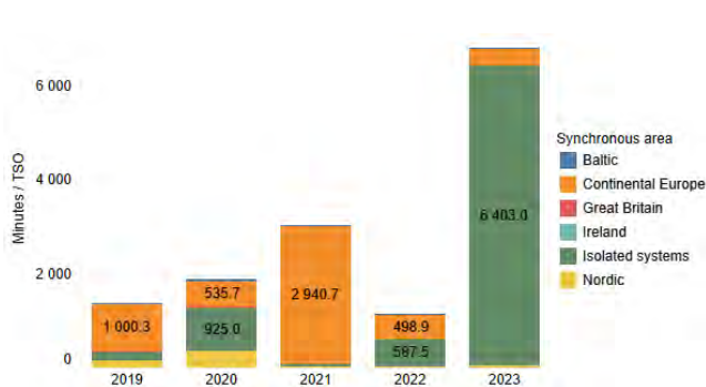
Figure 5.4: Operational security indicator OS-D1 from 2019–2023. It is calculated by adding up the number of minutes in alert and emergency states of all reported scale 0–3 incidents, and dividing by the number of TSOs in the synchronous area.
